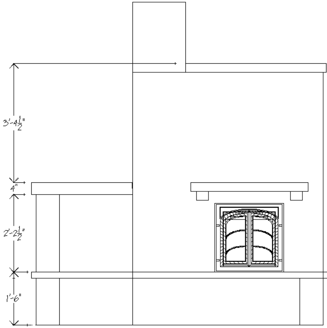
Figure 3. Front Elevation
