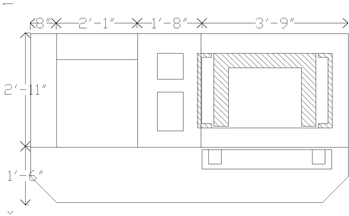
Figure 4. Plan
