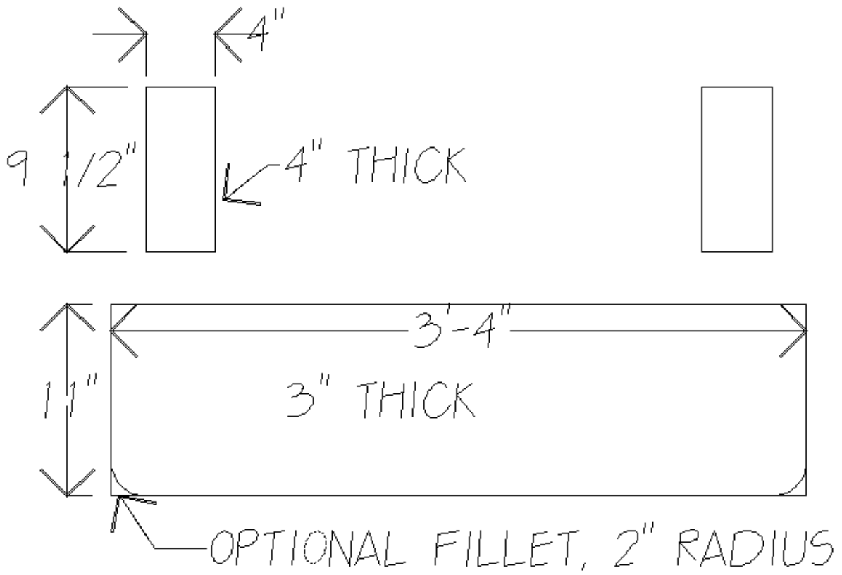
Figure 10. 3" Marble Slabs for Mantle
