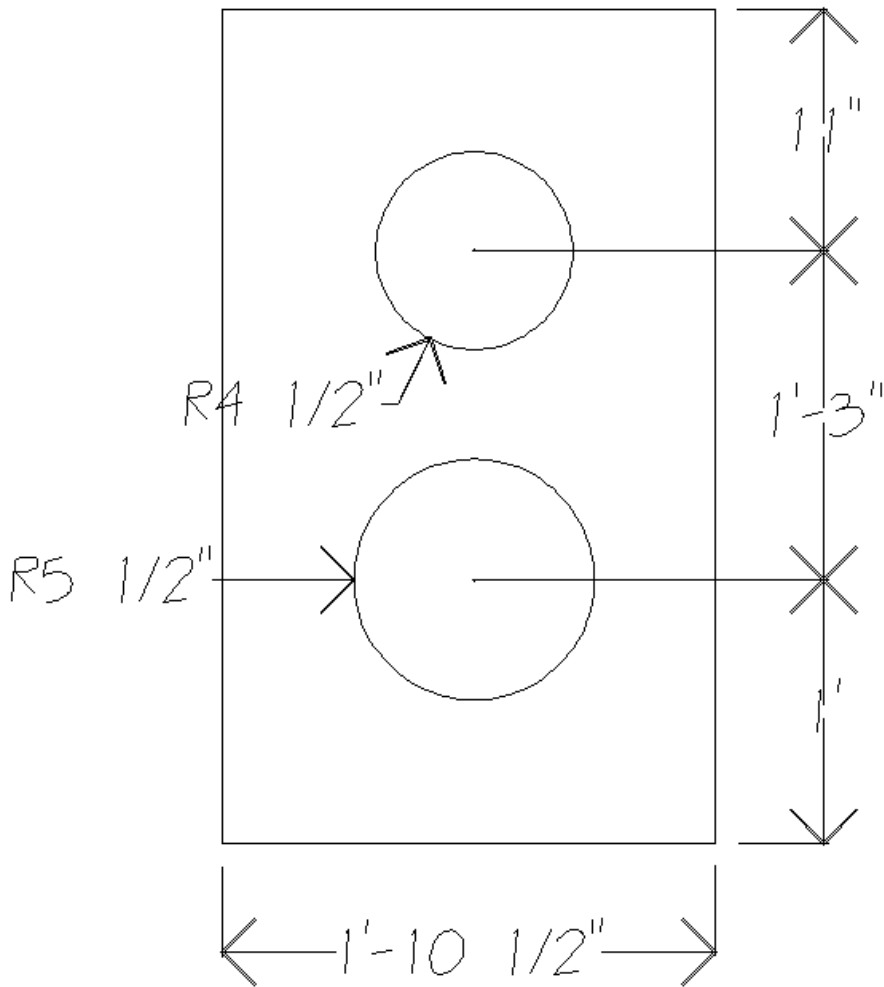
Figure 8. 3" Marble Slabs to Cap Heated Bench
