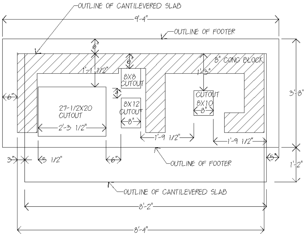
Figure 5. Foundation
