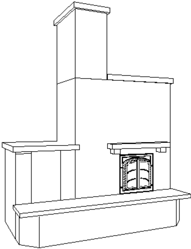
Figure 11 . Perspective Showing Slabs (Heated bench not as built)
