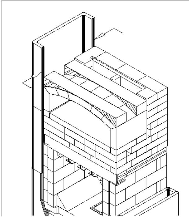
Figure 49 Height adjustment
