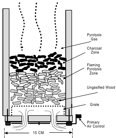
Fig. 1-Natural convection gasifier stove made with 15 cm riser sleeve 2,3
