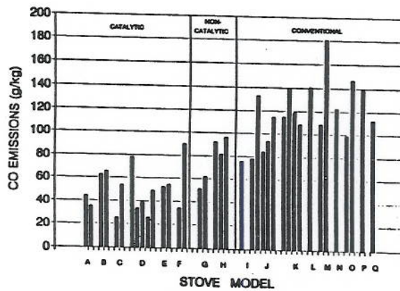
Fig. 10. Average CO emission factors of stoves in Crested Butte.
