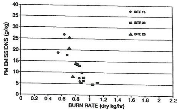
Fig. 5. PM emissions of noncatalytic model H stoves in Crested Butte.
