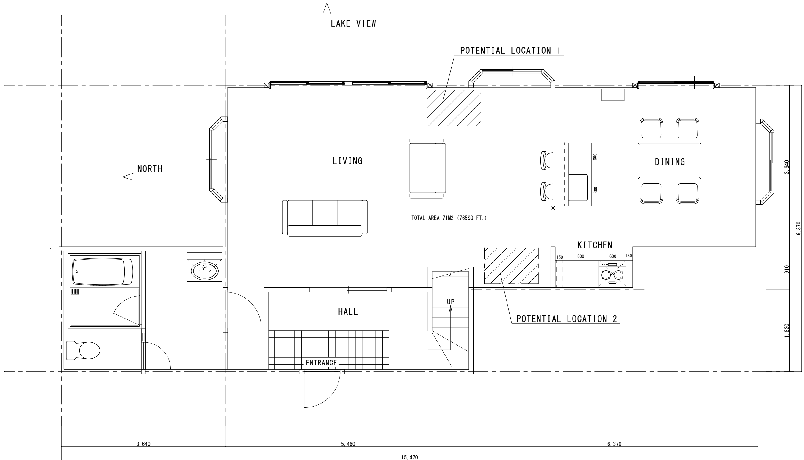
AKI'S WEEKEND HOME IN NAGANO 1ST FLOOR
